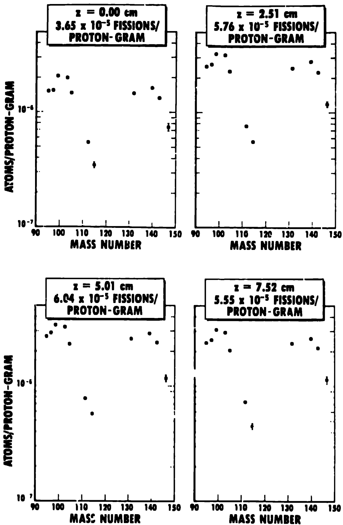
Fig. 6. Measured production of various atoms as a function of target axial position. The position z = 0.00 cm is the front target face where the ^{235}\text{U} - ^{235}\text{U} protons were incident.
