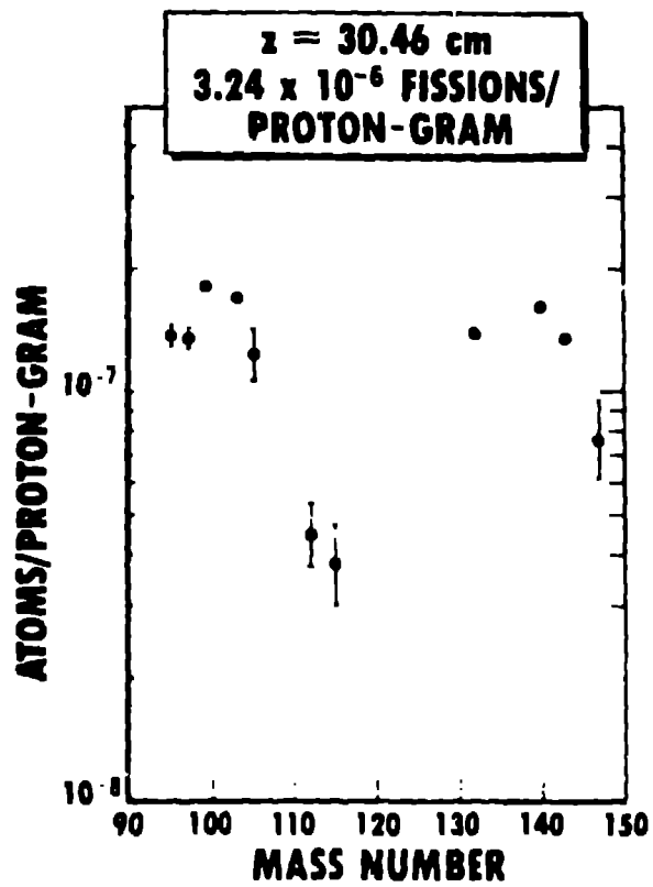
Fig. 8. Measured production of fission products as a function of fission product mass number. The position z = 30.46 cm is the front target face when the ^{235}\text{U} products were analyzed.
