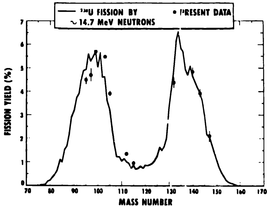
Fig. 10. Fission yield versus mass number for ^{235}\text{U} fission by 14.7 MeV neutrons.
