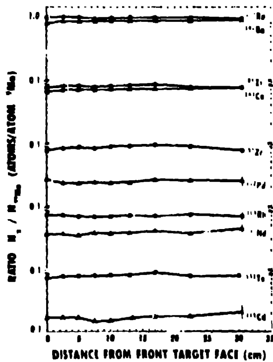
Fig. 9. Ratio of measured fission product formation to that of ^{99}\text{Mo} as a function of target axial-position.
