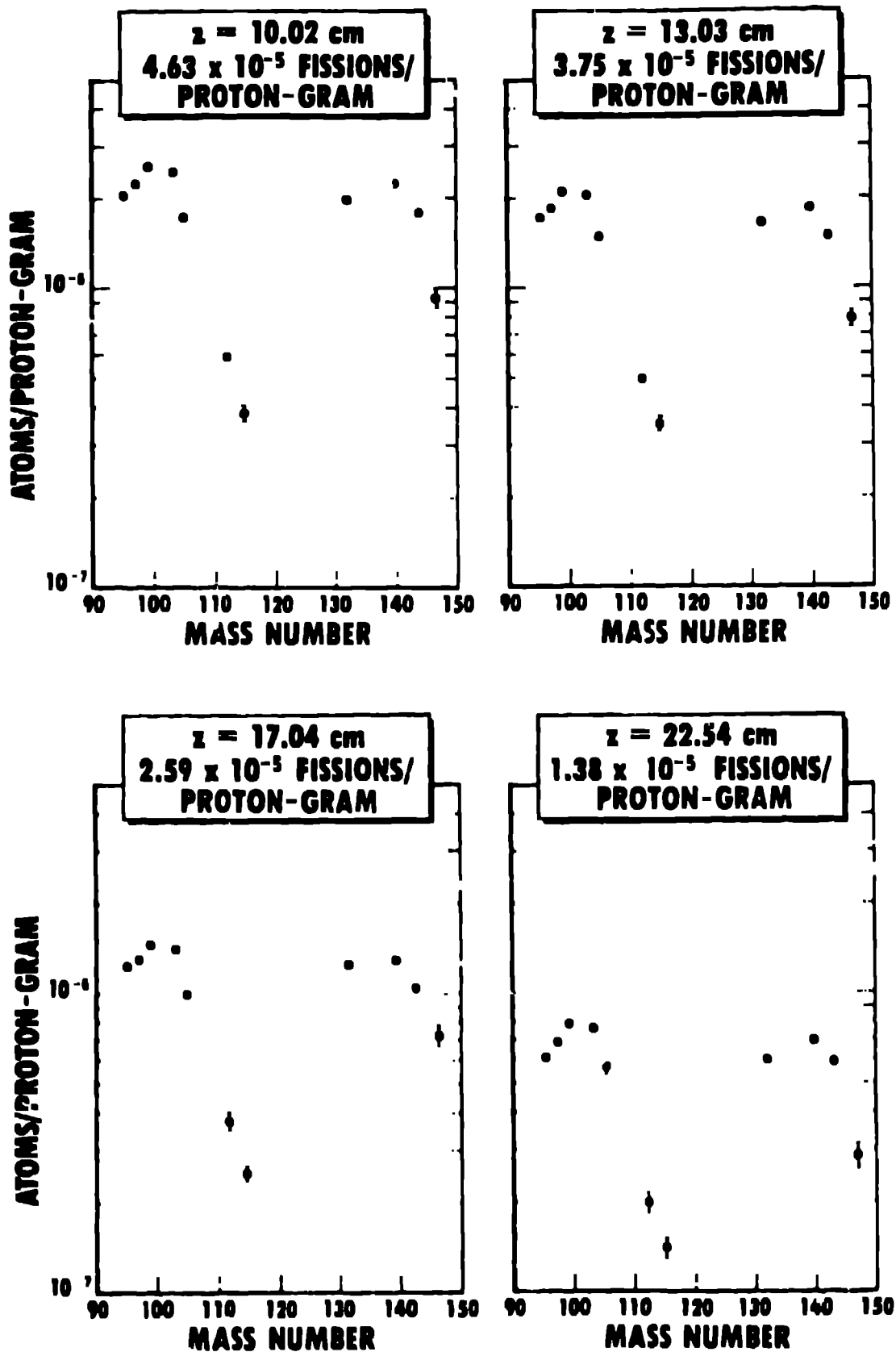
Fig. 7. Measured production of various atoms as a function of target thickness and position. The position at z = 0.50 cm is the front target face where the ^{235}\text{U} protons were incident.
